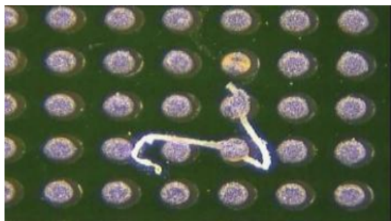
Lint contamination
